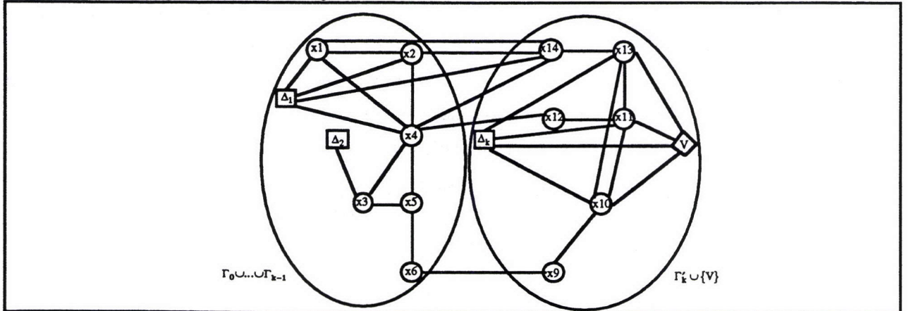
Figure 3. Moral graph without x_7 and x_8
