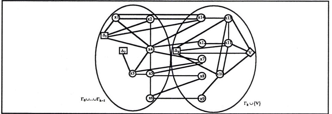
Figure 2. Moral graph with x_7 and x_8
